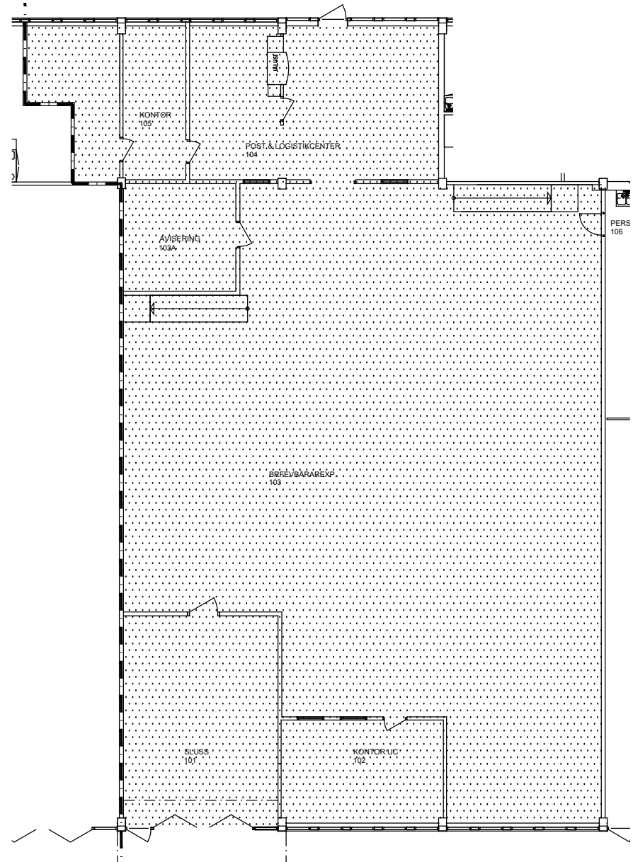
PLAN 1
